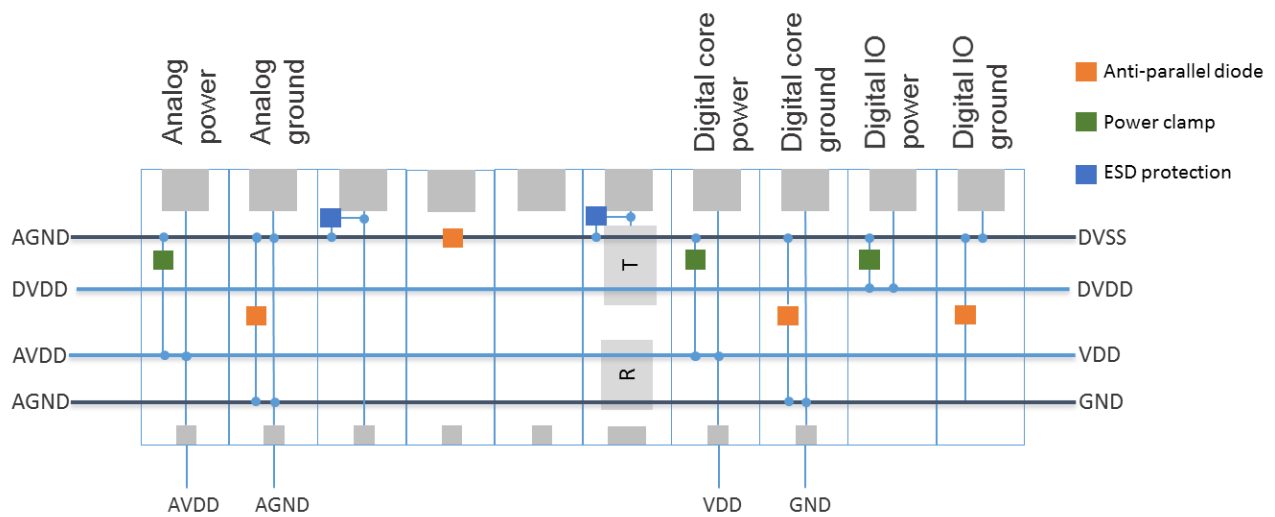
Figure 13.1 – GBT-SCA power distribution scheme
