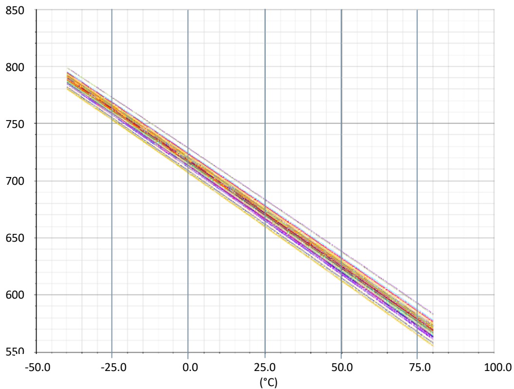
Figure 11.2 Temperature Measurement
