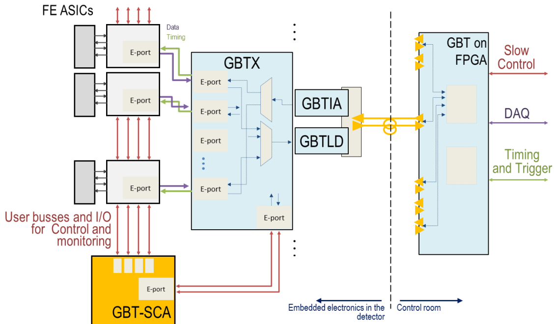
Figure 2 typical implementation of on-detector electronics making use of the GBT-chipset
