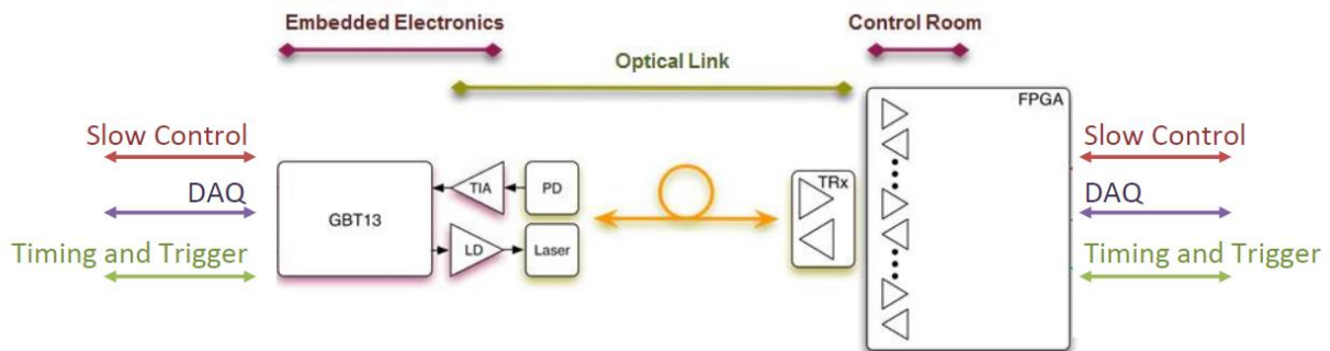
Figure 1 generic topology of the GBT system
