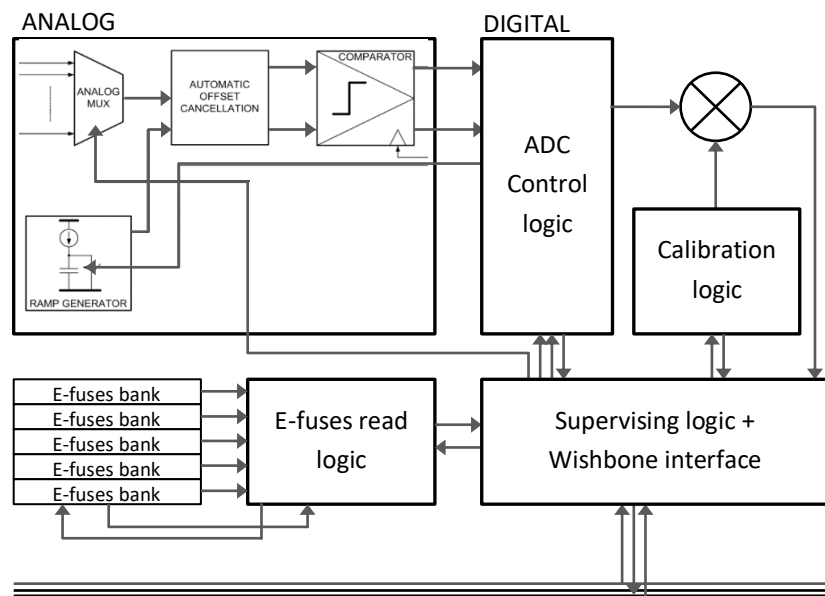
Figure 11.1 – Block diagram of the ADC channel
