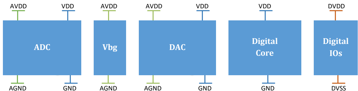
Figure 13.2 – GBT-SCA power supply connectivity
